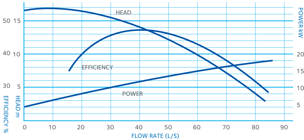
RH 7A 20 YARDMASTER PUMP - IMPELLER DIAMETER 229mm x 77mm
